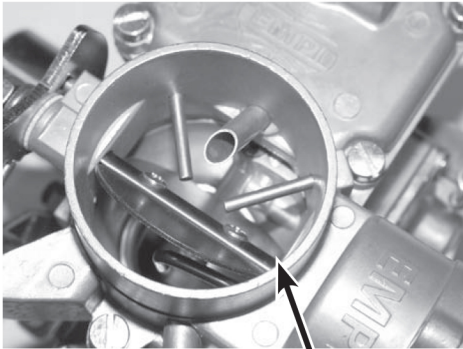
Choke is fully open
